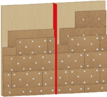
Double-course installation over solid wood
