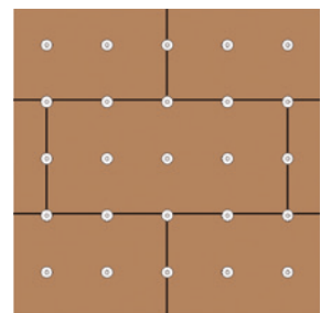
10 Fasteners/m 2
