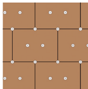
10 Fasteners/m 2
