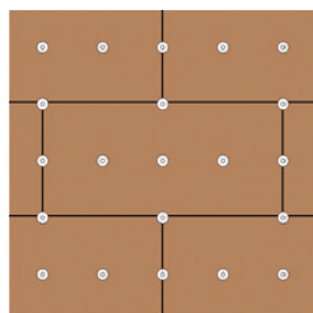
8 Fasteners/m 2
