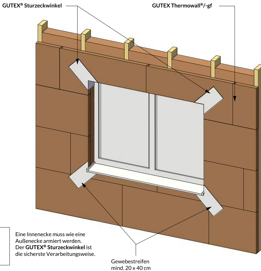
Window and door openings with diagonal reinforcement
